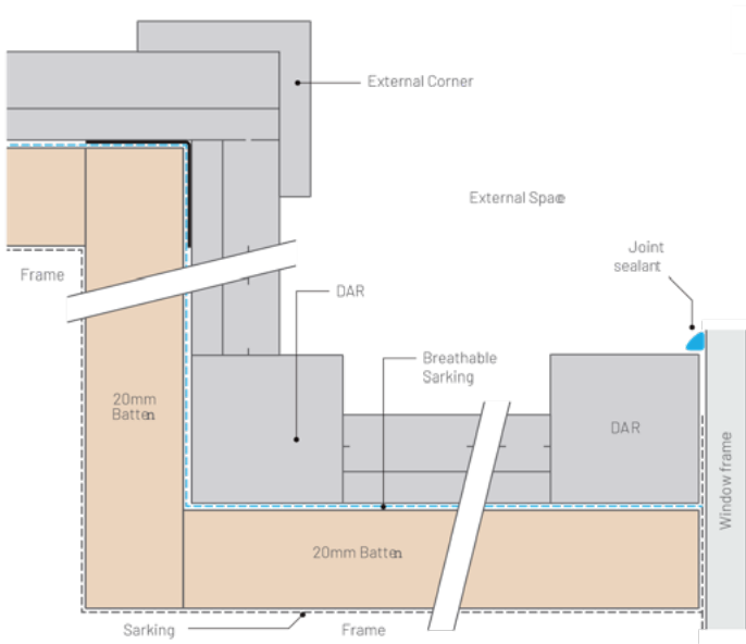
Internal / external stops (timber)
