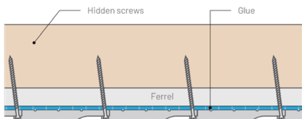
Horizontal installation - internal ceiling
