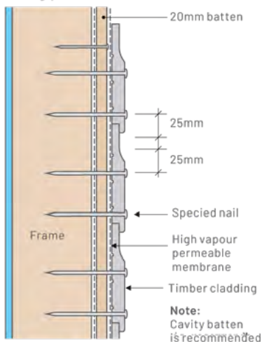
Horizontal installation - external
