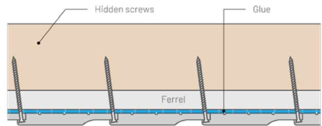
Horizontal installation – internal ceiling
