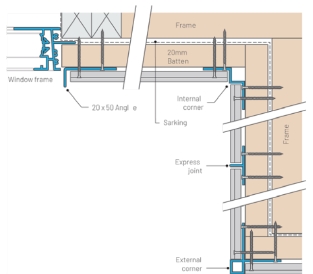
Hidden Interior / external stops (aluminium) extra detail
