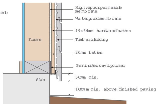
Minimum clearance level of cladding above final ground levels and finishing below bottom plate
