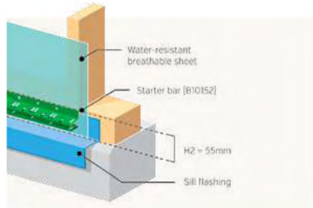
Outside corner
