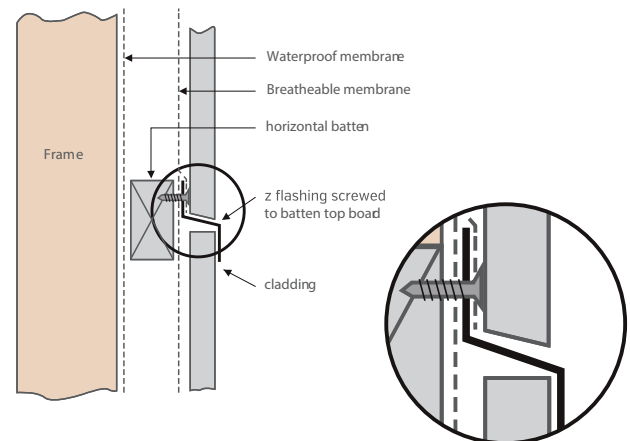
Vertical installation
