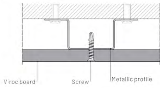
Detail B (steel structure) Board central zone
