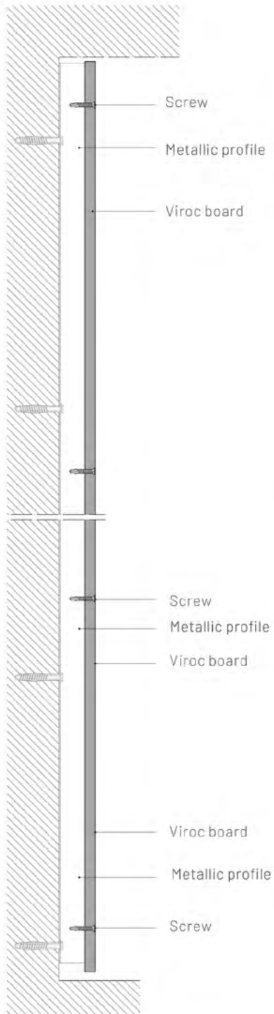
Steel structure
