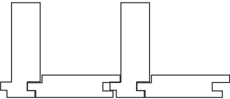
Step 27mmx67mm and Flat 81mmx17mm
