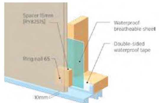
Lower part
