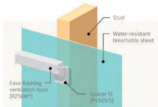
Eave
