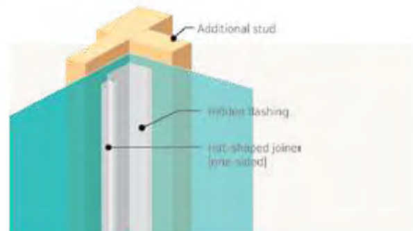
Inside corner
