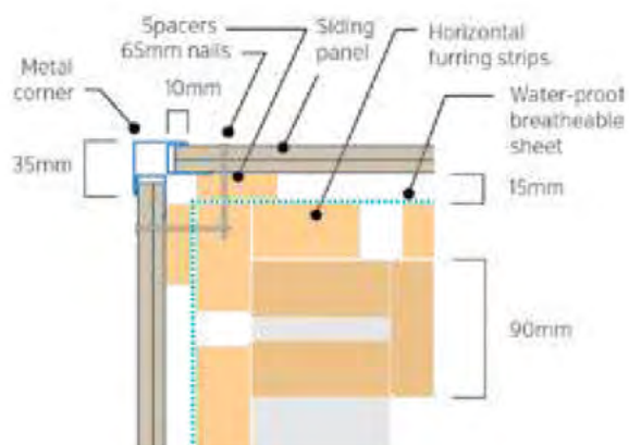
Corner siding
