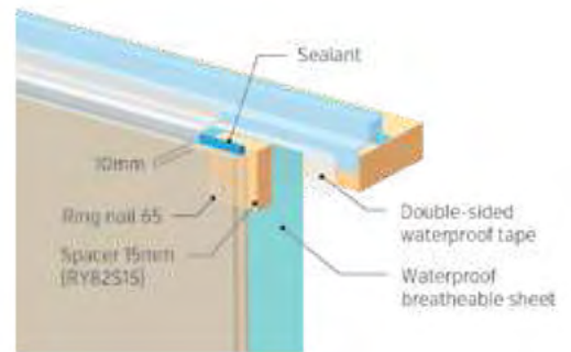
Upper part
