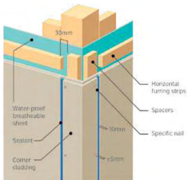
Corner siding
