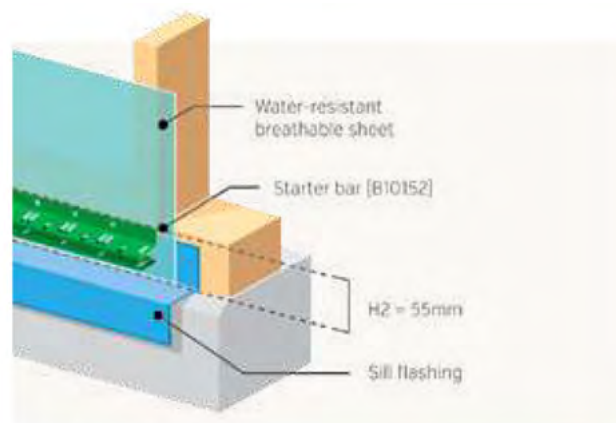
Outside corner
