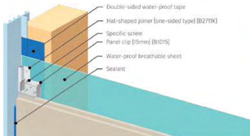
Sides
