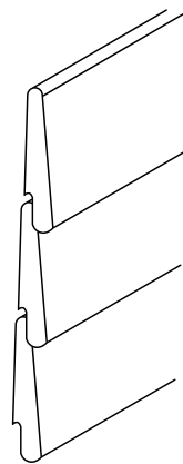
Horizontal Installation
