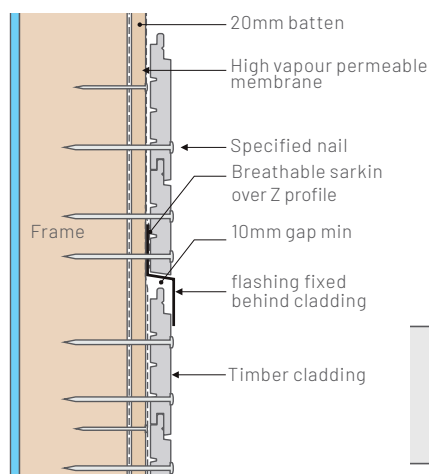
Face fixing showing fixing position
