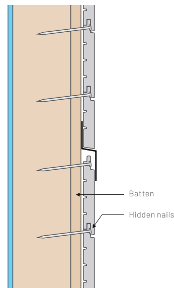
Horizontal installation - internal wall
