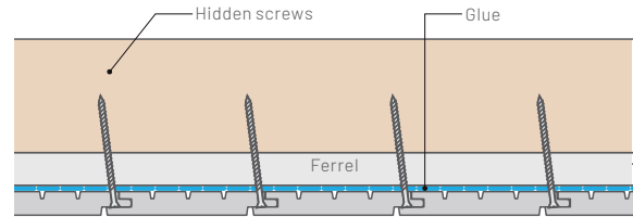
Horizontal installation - internal ceiling
