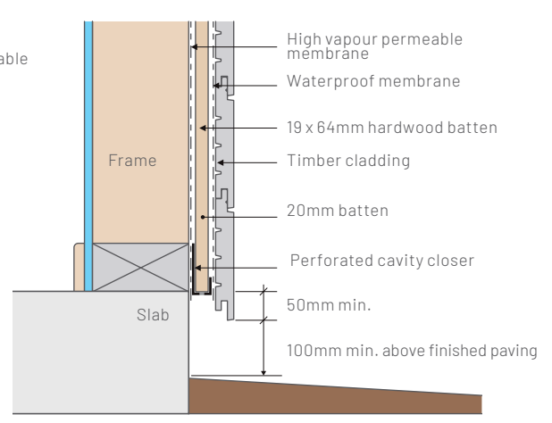
Minimum clearance level of cladding above final ground levels and finishing below bottom plate
