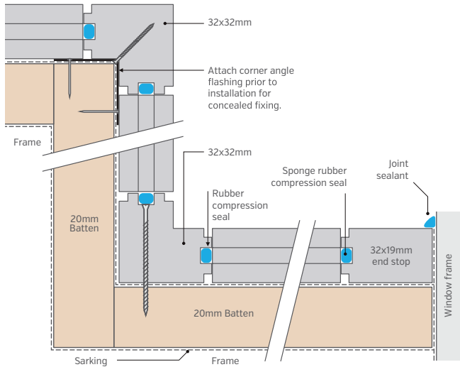
Internal / external stops (timber)
